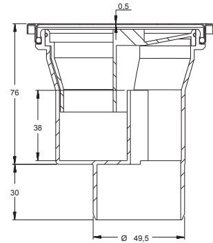
Ø 50 BOTTOM OUT
