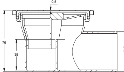
Ø 50 SIDE OUT
