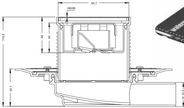
Ø 32 Side Out
